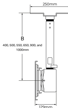
SIDE MOUNTING
