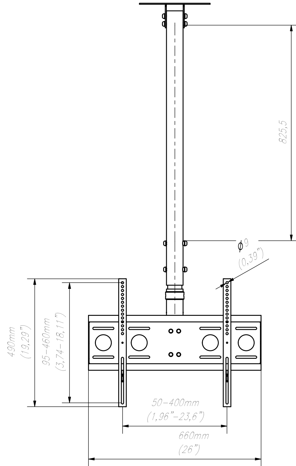
FRONT VIEW
