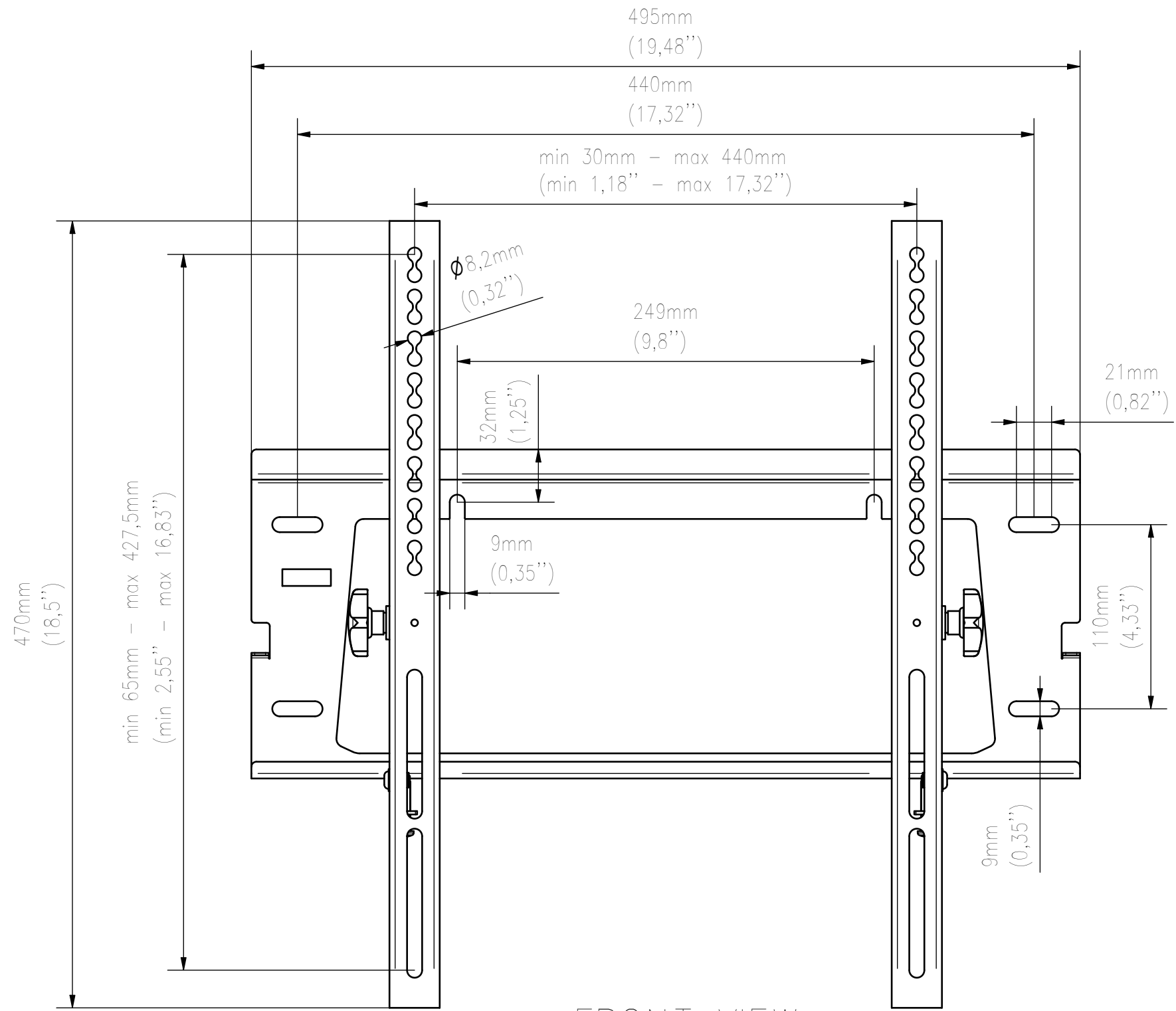
FRONT VIEW
