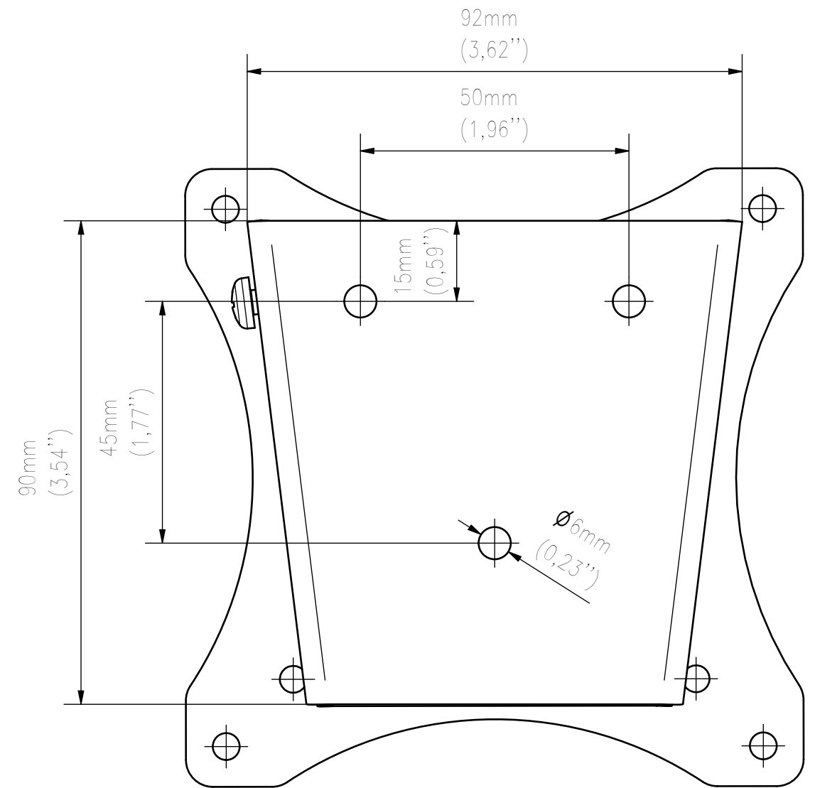
BACK VIEW
