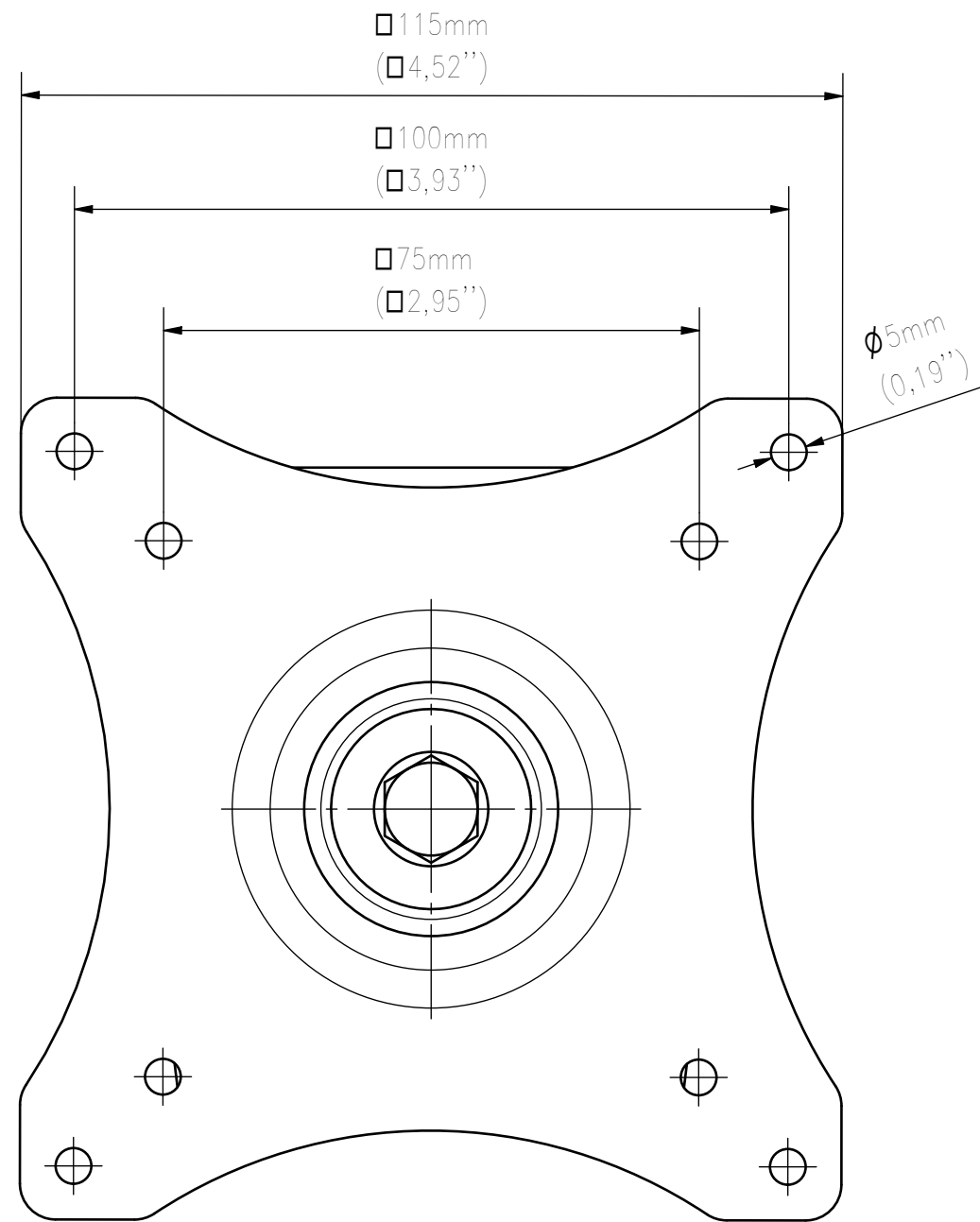
FRONT VIEW
