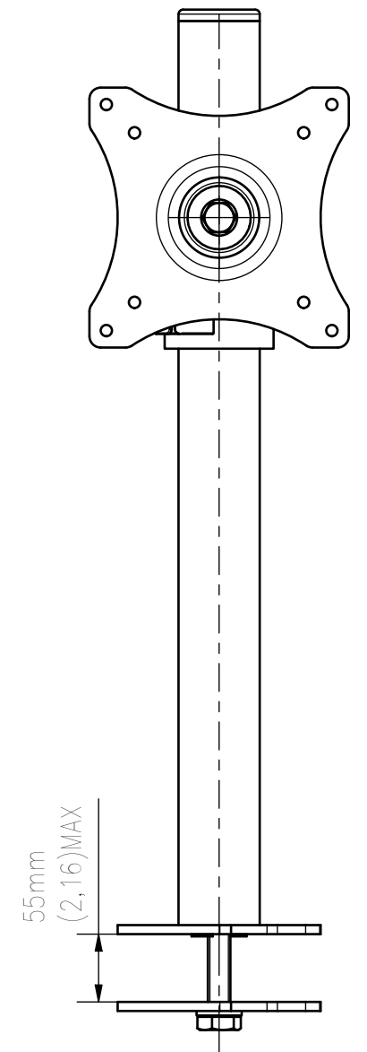
FRONT VIEW
