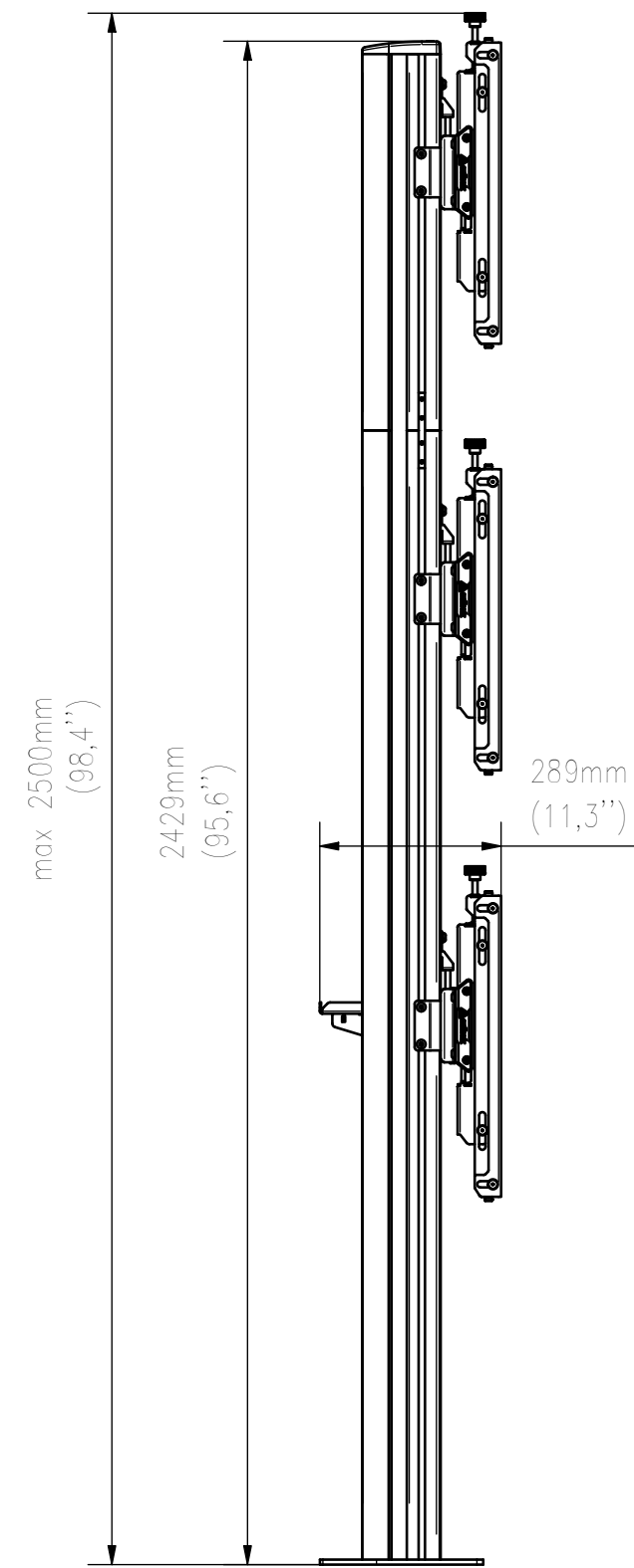
SIDE VIEW
