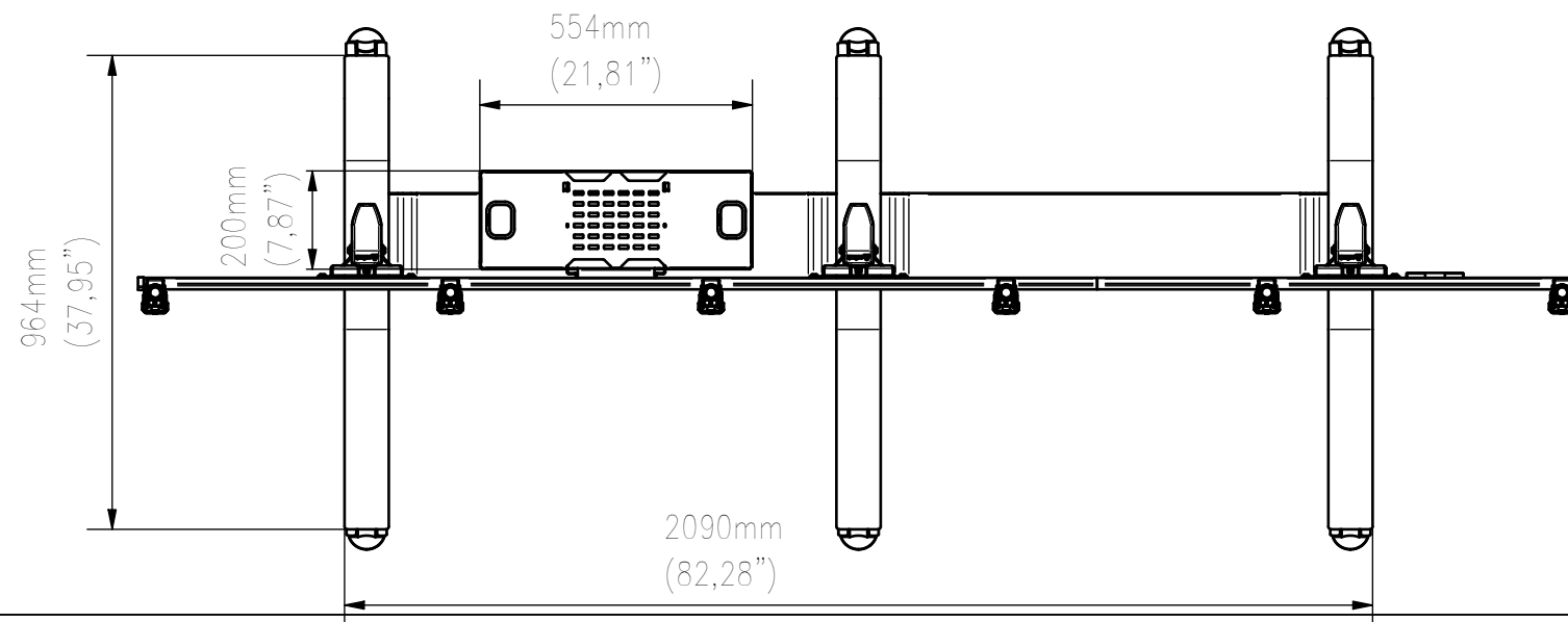
TOP VIEW
